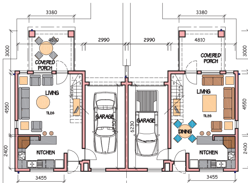
F GROUND STOREY PLAN Fm
