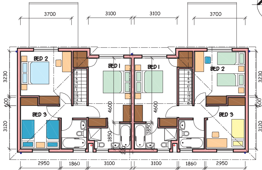
F FIRST STOREY PLAN Fm
